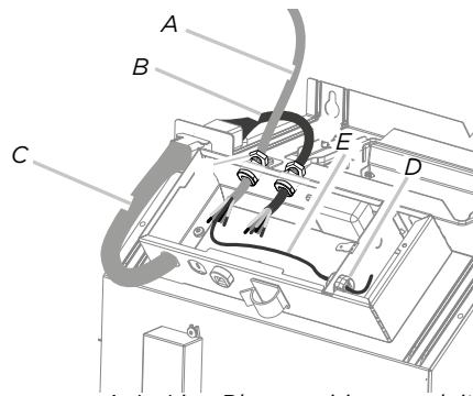
A. In-Line Blower wiring conduit (not included) B. 6-9 wire connector C. Hood Insert Blower Connector D. Range Hood strain relief E. Strain relief
