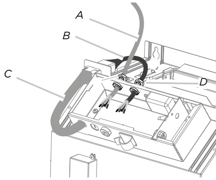
A. In-Line Blower wiring conduit (not included) B. 6-9 wire connector C. Hood Insert Blower Connector D. Strain reliefs
