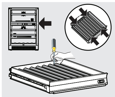
Dual Zone Shelf Removal
