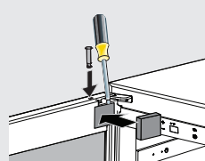
Hinge pin/hinge pin retainer
