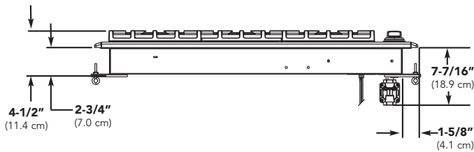
VGSU Front View
