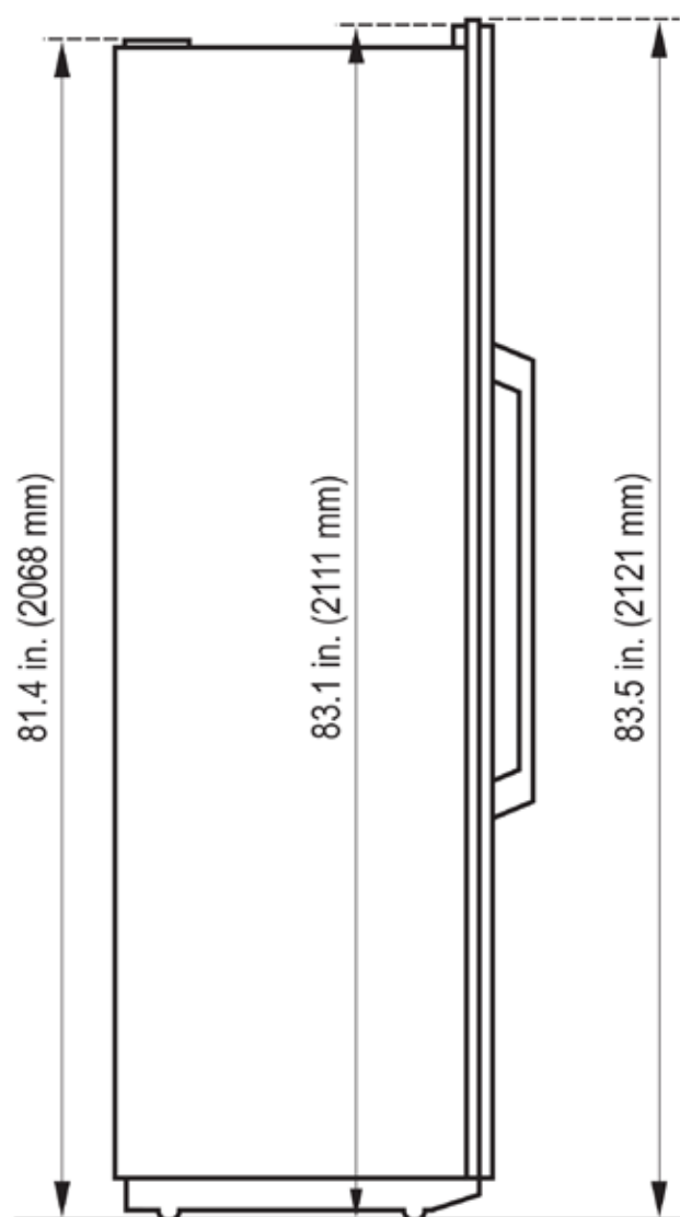
Left View
