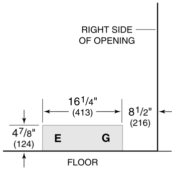
Gas Supply Illustration
