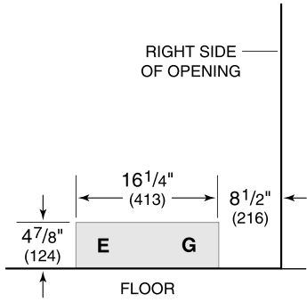
Electrical Location Illustration
