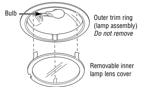
Use a small flat blade screwdriver to remove the inner lamp lens cover.
