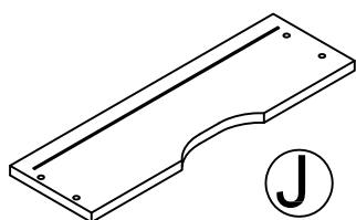
DRAWER FRONT T1323015100CS QTY: 2PCS
