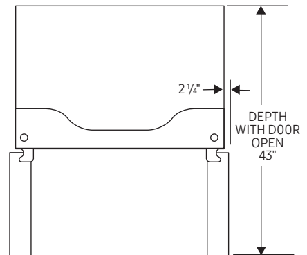
TOP OF REFRIGERATOR WITH DOORS OPEN 90°
