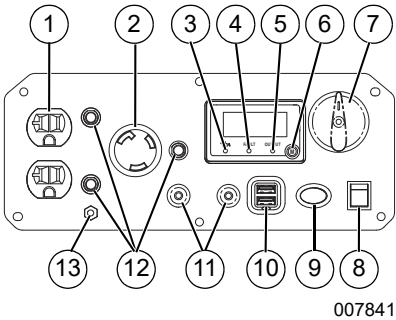
Figure 2-2. Control Panel
