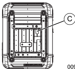
Figure 4-4. Remove Oil Drain Rubber Cover
