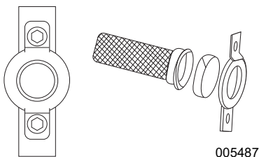
Figure 4-8. Spark Arrestor Screen
