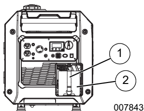
Figure 2-8. Battery Connection
