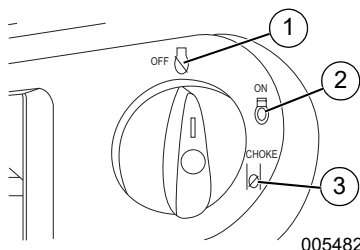
Figure 2-6. Switch (example)
