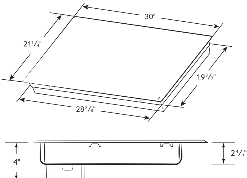
Cooktop Dimensions
