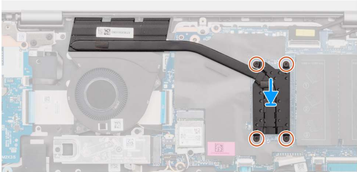
Figure 41. Installing the heat sink - for computers shipped with integrated graphics card
