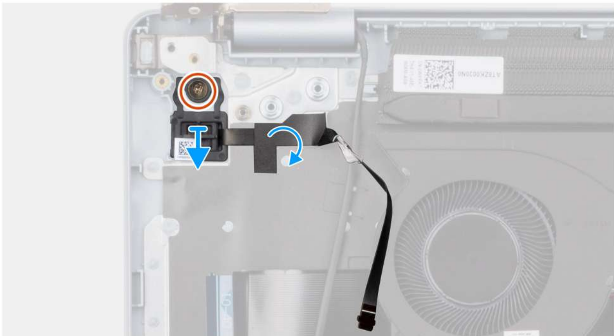
Figure 74. Removing the power button with fingerprint reader
