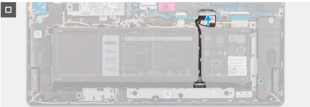
Figure 36. Connecting the battery cable
