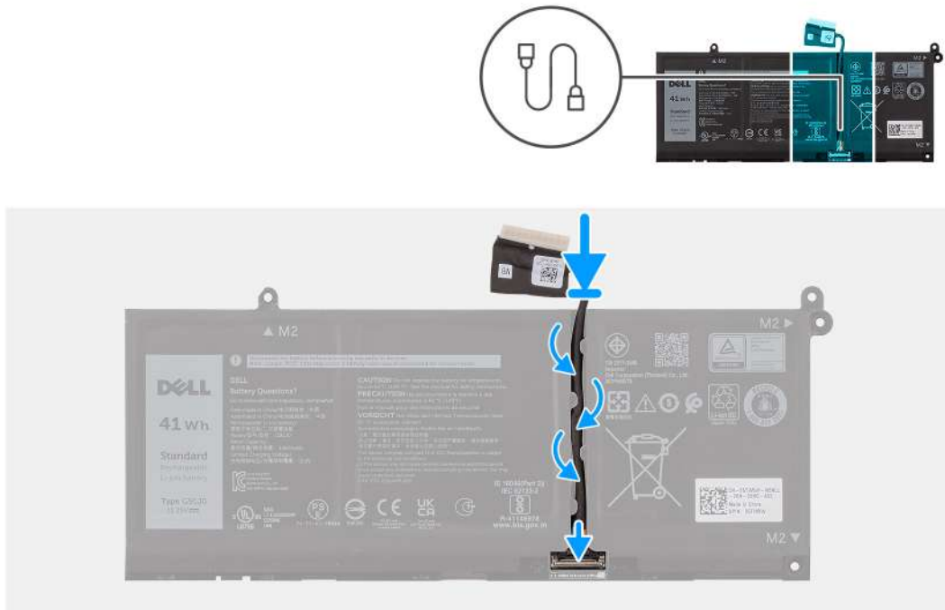
Figure 25. Connecting the battery cable
