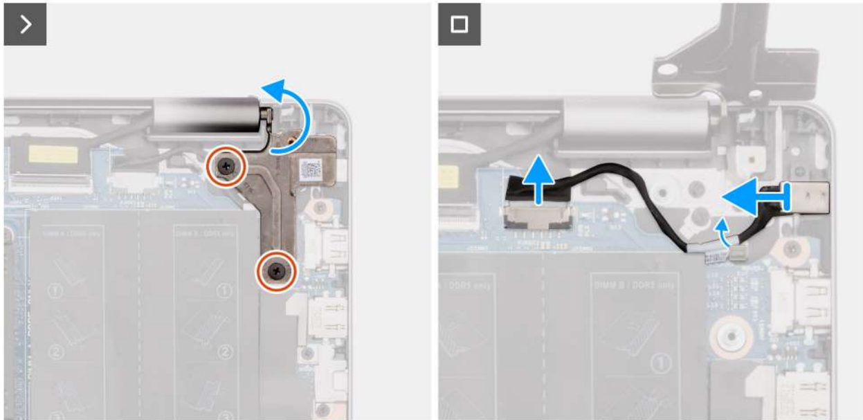
Figure 77. Removing the power-adapter port
