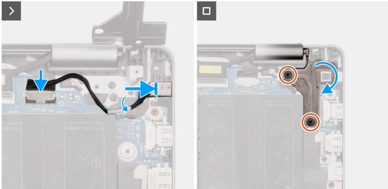
Figure 78. Installing the power-adapter port
