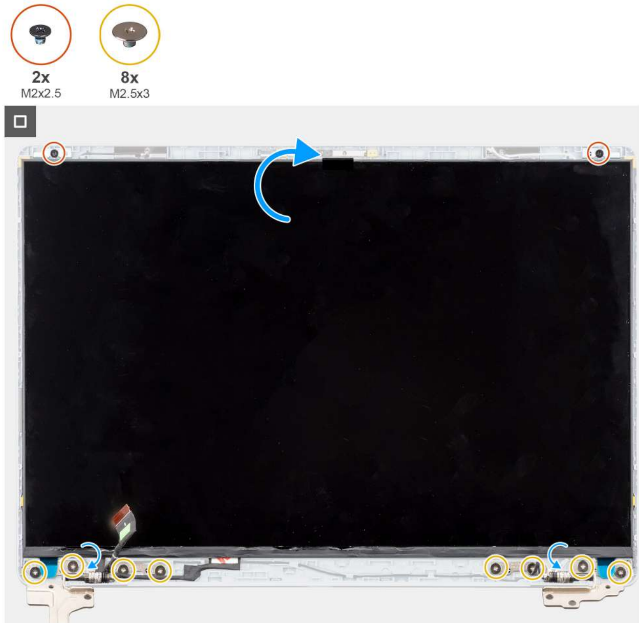
Figure 65. Installing the display panel
