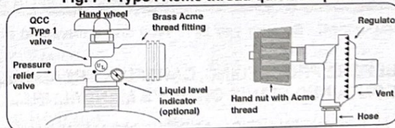
Fig. 7-1 Type I Acme thread quick coupler
