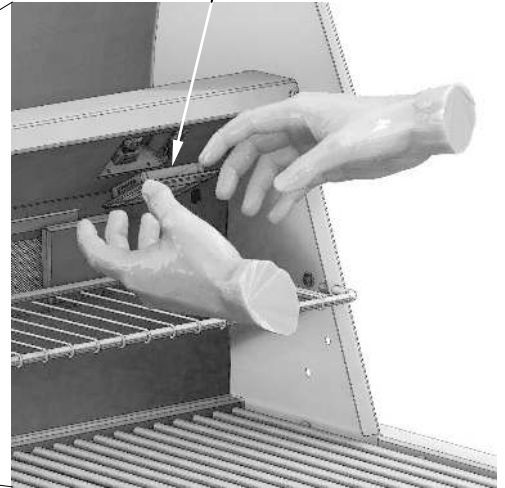
LIGHT COVER
