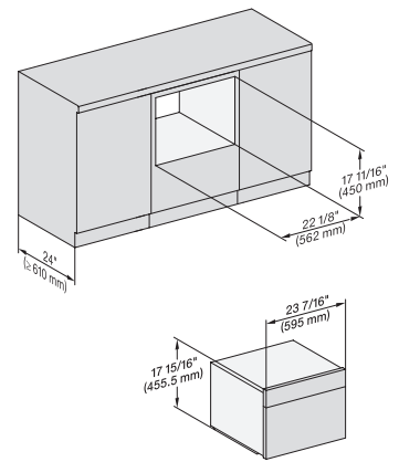
installation Proud built-under 450S, installation drawing, NA
