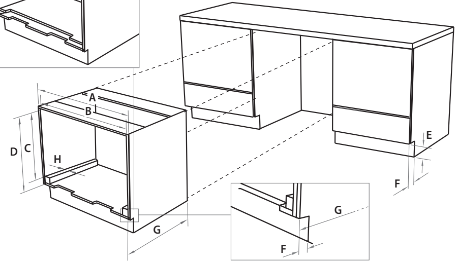
Cabinetry dimensions (mm)
