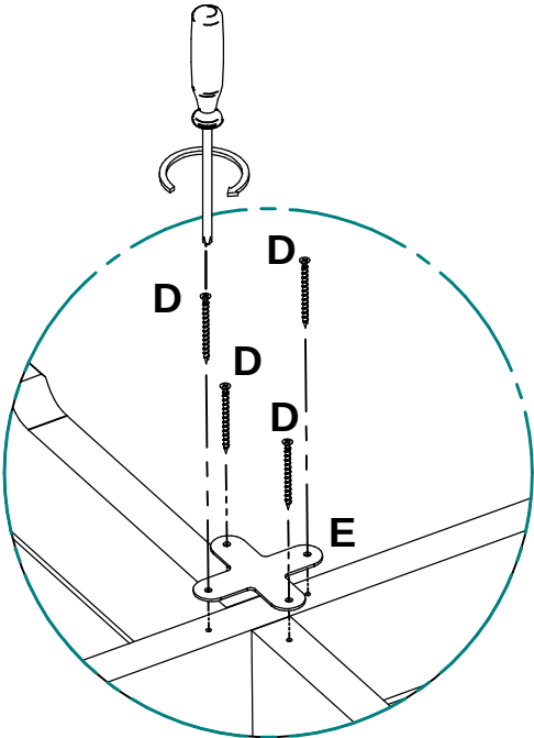
DETAIL C
