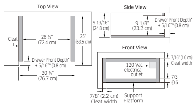
FLUSHED CABINET DIMENSIONS
