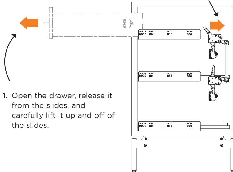
REMOVING THE FIRST DRAWER
