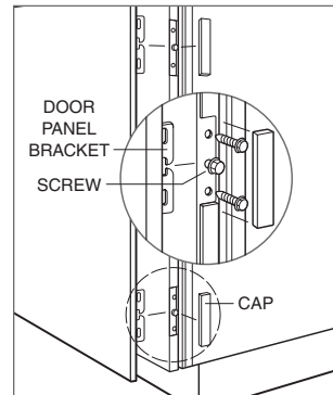
Panel installation.
