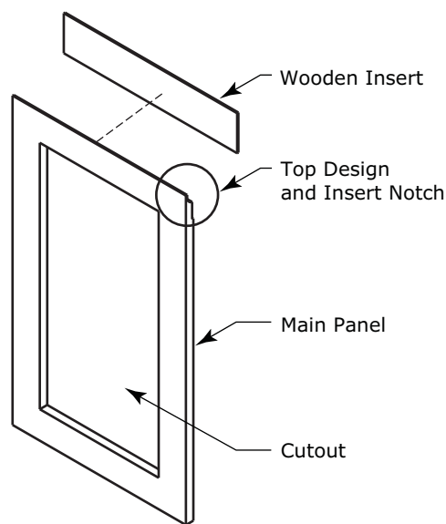
Integrated Frame
