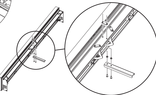
Figure 12. Dual Grille Slide Bracket Installation
