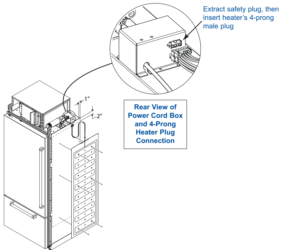
Figure 1. Heater Installation
