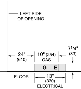
Gas Supply Illustration
