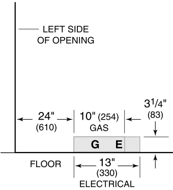
Electrical Location Illustration
