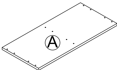
TOP T1748899010CS
