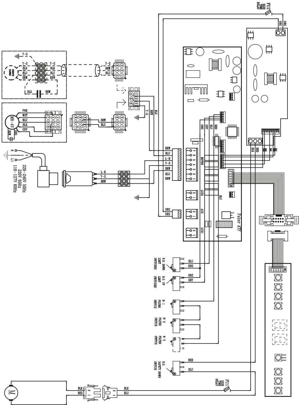
Downdraft unit wiring diagram
