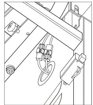
Connector housing
