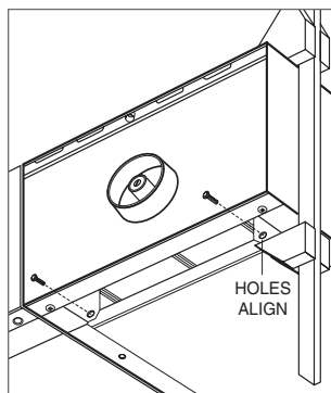
Hole alignment
