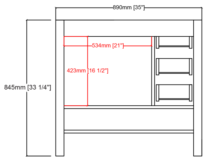
BACK VIEW
