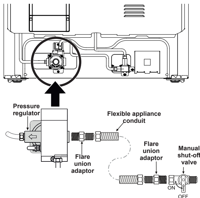
Fig. 8 - gas supply connections
