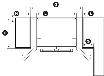
Flush with refrigerator door - full door rotation
